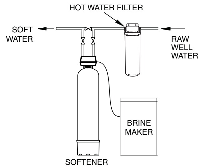
Figure 1. INSTALLATION SCHEMATIC
