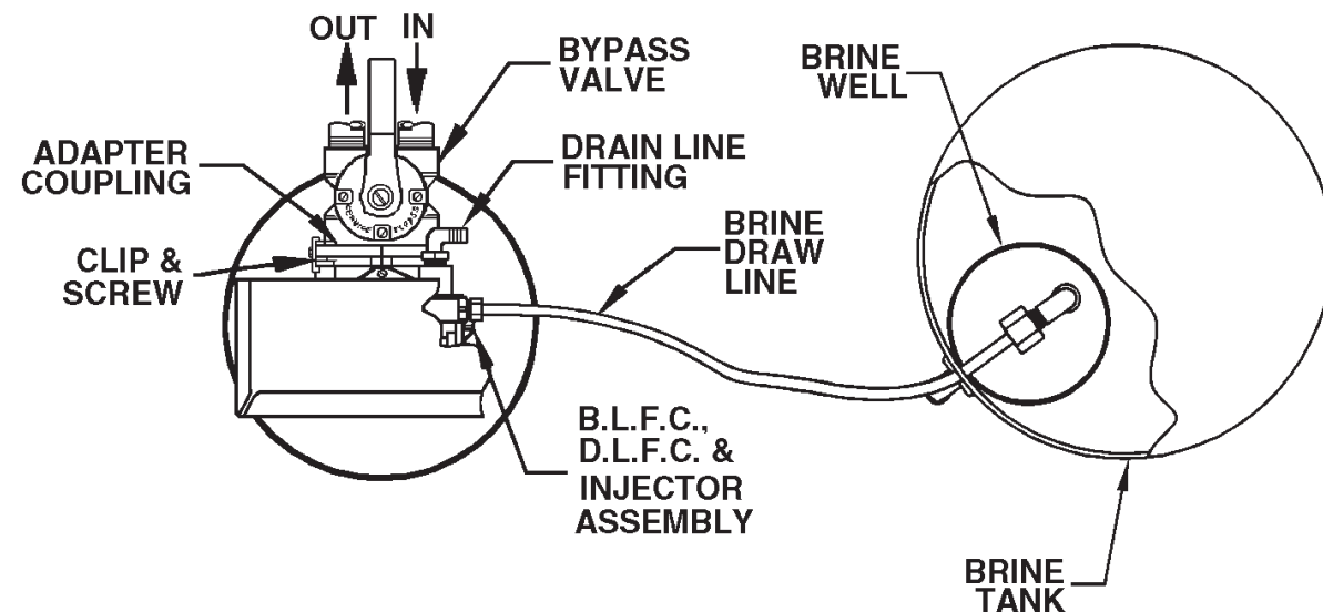
Figure 2. SOFTENER AND BRINE TANK ASSEMBLY, TOP VIEW
