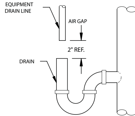
Figure 3. TYPICAL DRAIN
