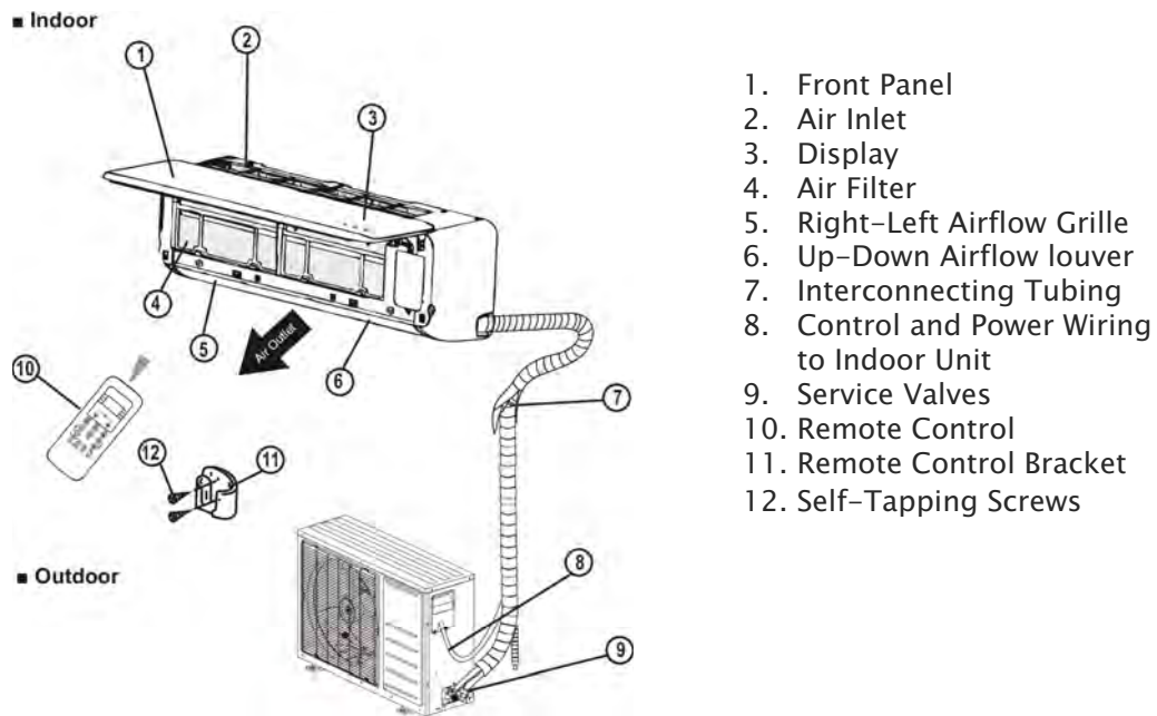
Fig. 1 — Indoor/Outdoor Unit
