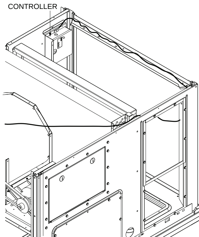
Fig. 8 — Controller Mounting Location
