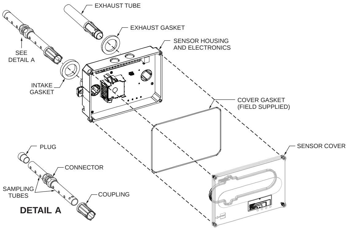
Fig. 2 — Smoke Sensor Exploded View
