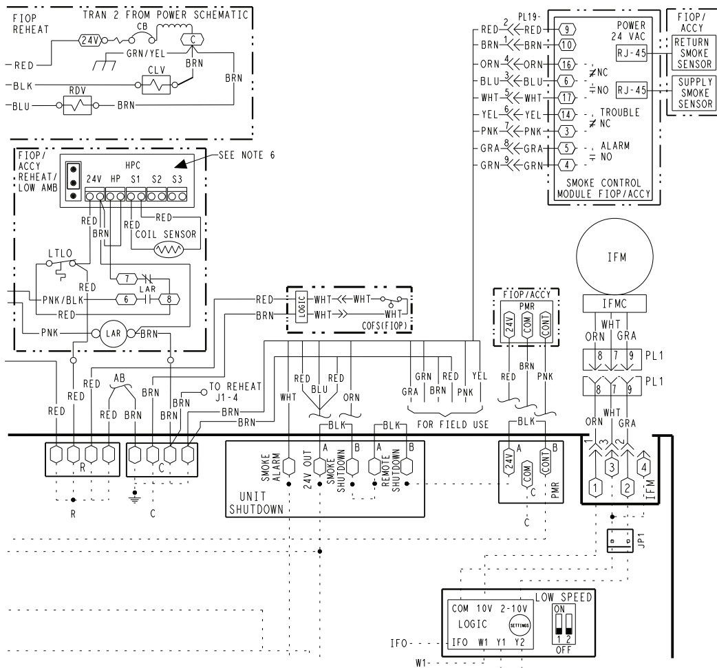
Fig. 7 — Smoke Detector Wiring
