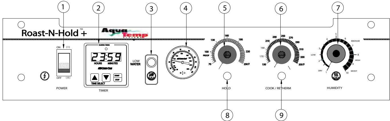
FIGURE 3: Control Panel
