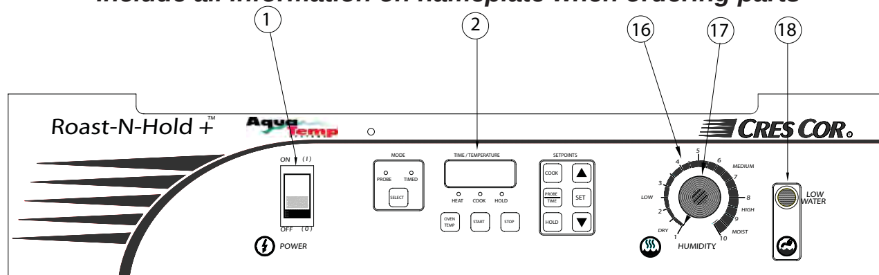
FIGURE 2: CONTROL PANEL
