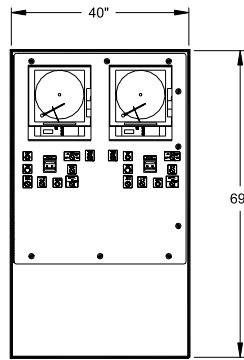
HA-DE-CC2 DUAL CONTROL PANEL
