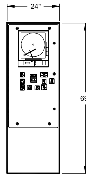
HA-SE-CC2 SINGLE CONTROL PANEL
