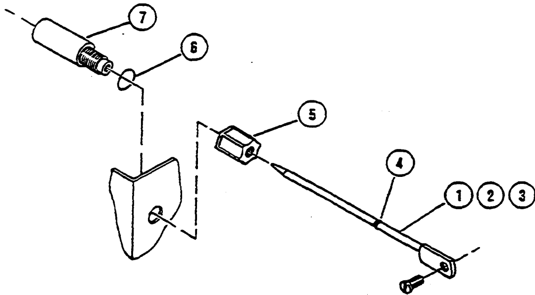
Fig. 9 PROBE ASSEMBLY
