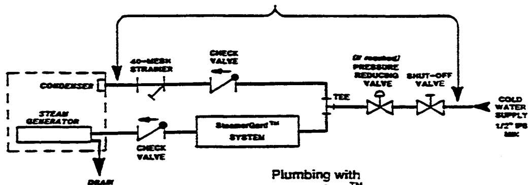
RECOMMENDED PLUMBING
