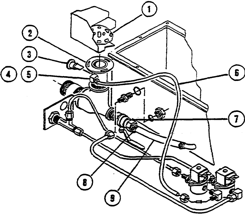
Fig.21 DRAINAGE SYSTEM
