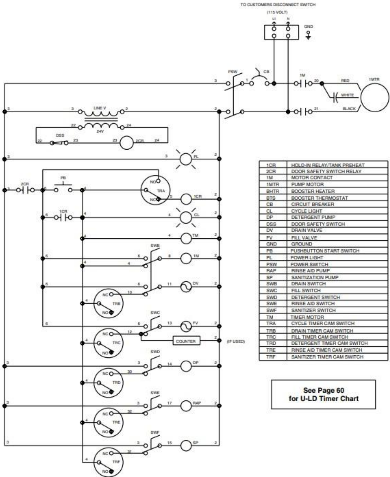
Figure 27 - U-LD Electrical Schematic
