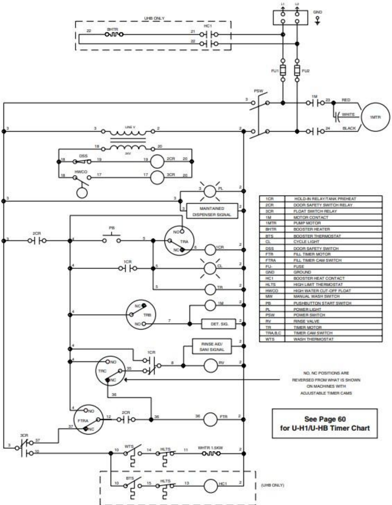
Figure 26 - U-H1/U-HB Electrical Schematic
