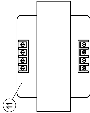
Main Power Transformer mounted on machine base
