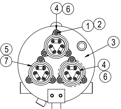
BOOSTER ASSEMBLY, 16kW @ 480V/60/3, 575V/60/3 (Right-to Left) (70°F/39°C Rise)
