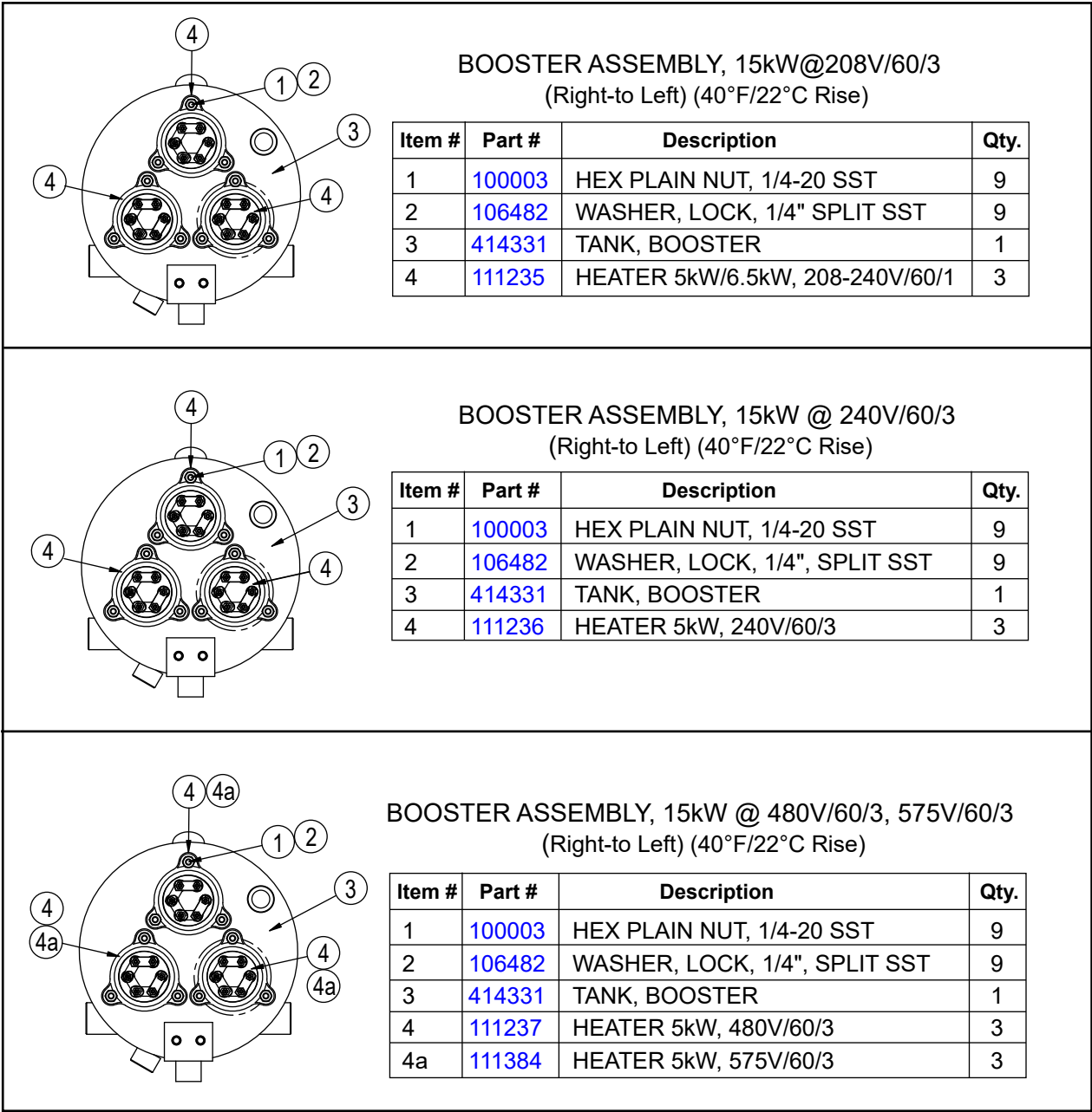
Figure - 20 (Parts List)
