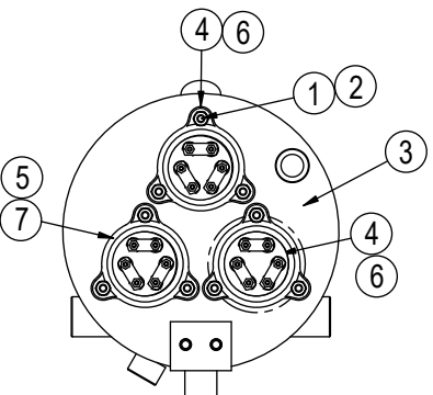
BOOSTER ASSEMBLY, 32kW @ 480V/60/3, 575V/60/3 (Right-to Left) (70°F/39°C Rise)
