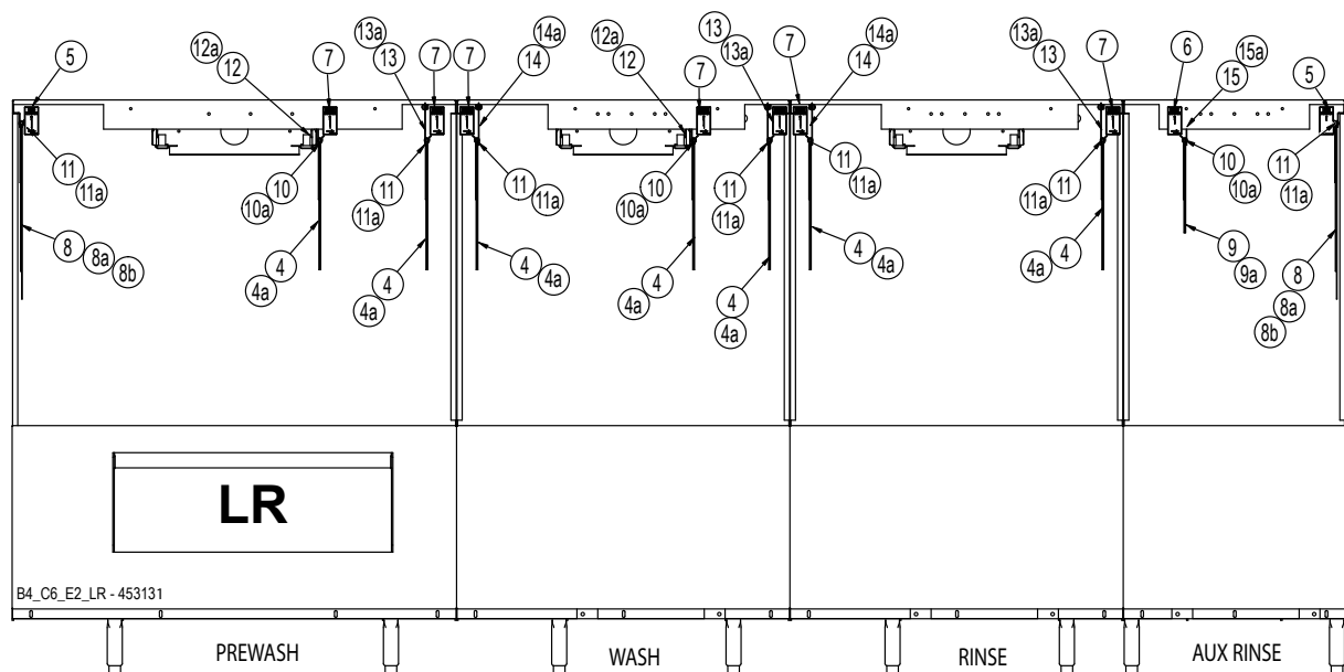
Figure - 90 (Parts List)
