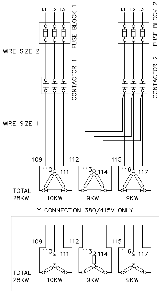
3 PHASE CONNECTION
