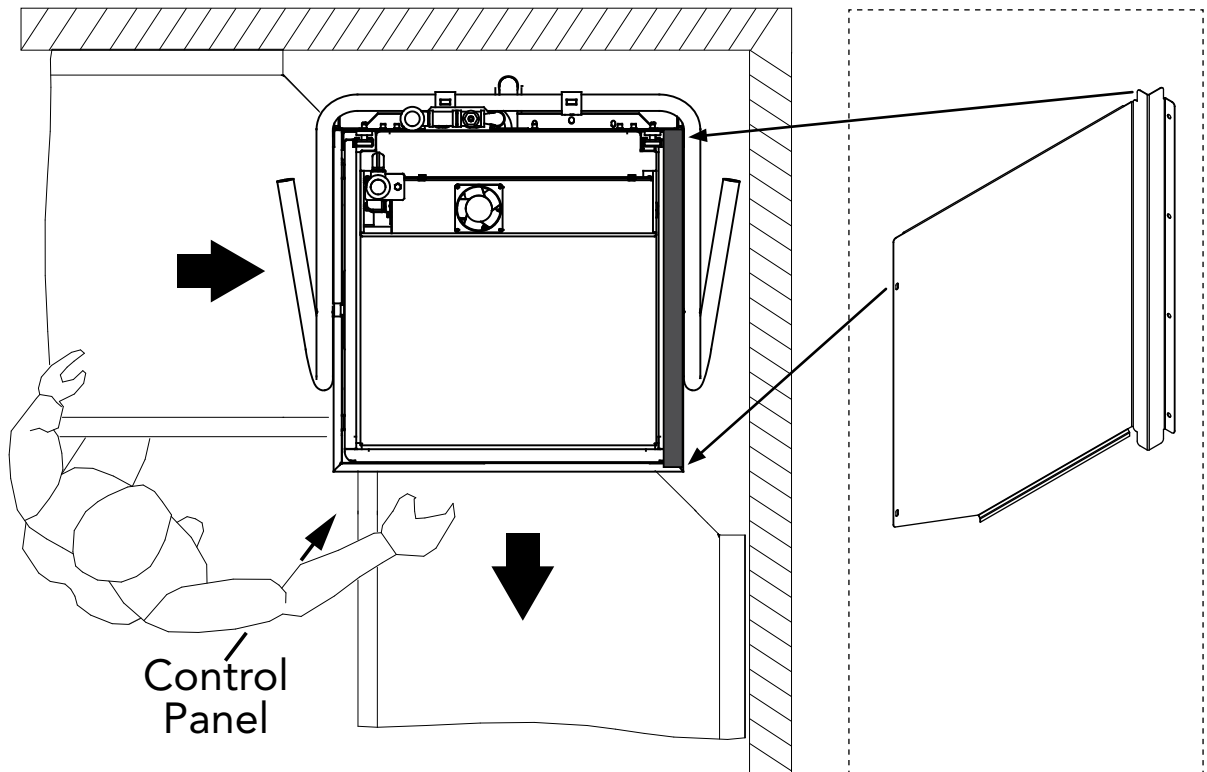
Fig. 4 - Nominal corner installation
