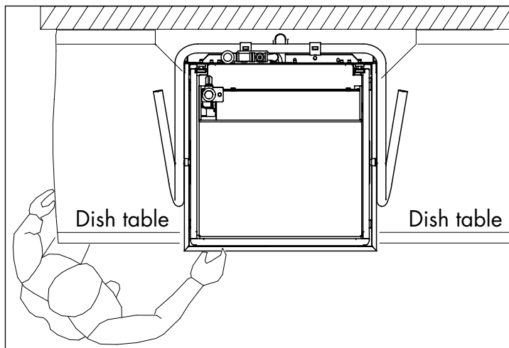
Fig. 3 - Nominal dish table configuration
