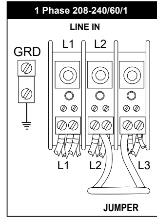
Fig. 15 - Jumper wire
