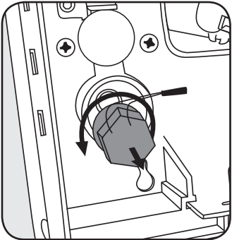
5. Unscrew and remove solenoid.
