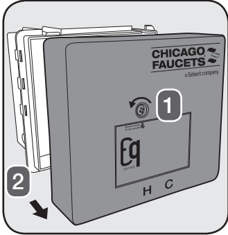
2. Loosen the cover screw with #2 Phillips screwdriver and remove control box cover.
