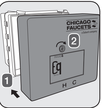
11. If all is good, reinstall the control box cover and secure it with the #2 Phillips screw.
