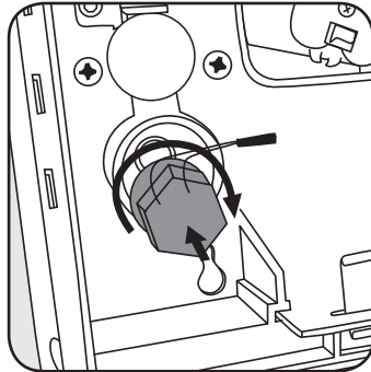
6. Install new solenoid. Hand tighten.
