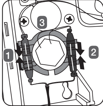
9. Reconnect the wiring connectors (gray to gray, black to black). Note that the connectors are keyed for proper installation as shown in the detail below. Snap the completed connections, into the wiring harness as shown.
