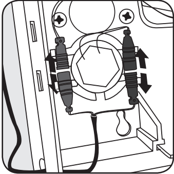
3. Disconnect power and solenoid.
