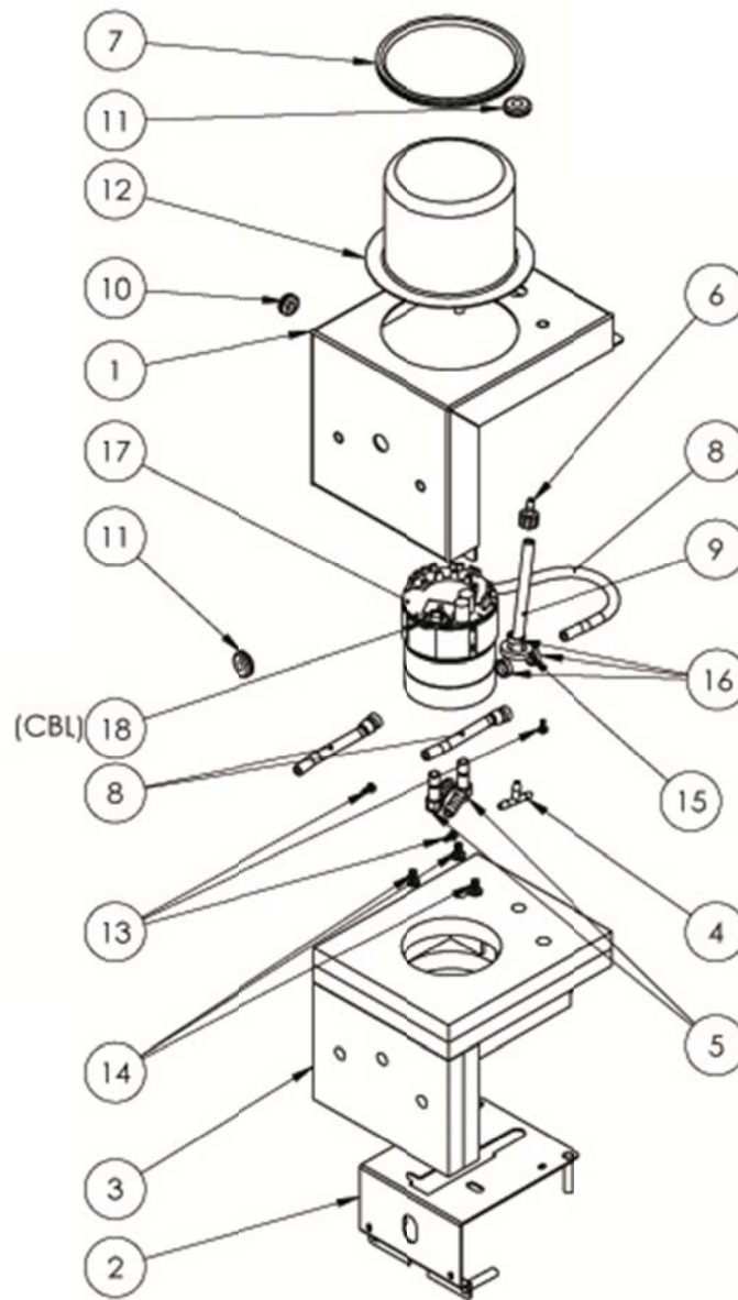
Diagram 16: Milk Pump Assembly
