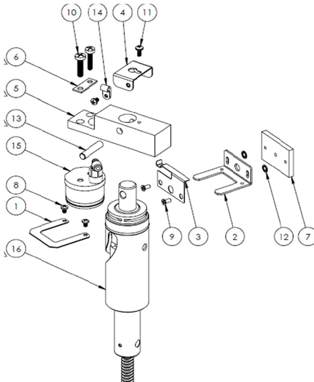
Diagram 12: Upper Piston XT
