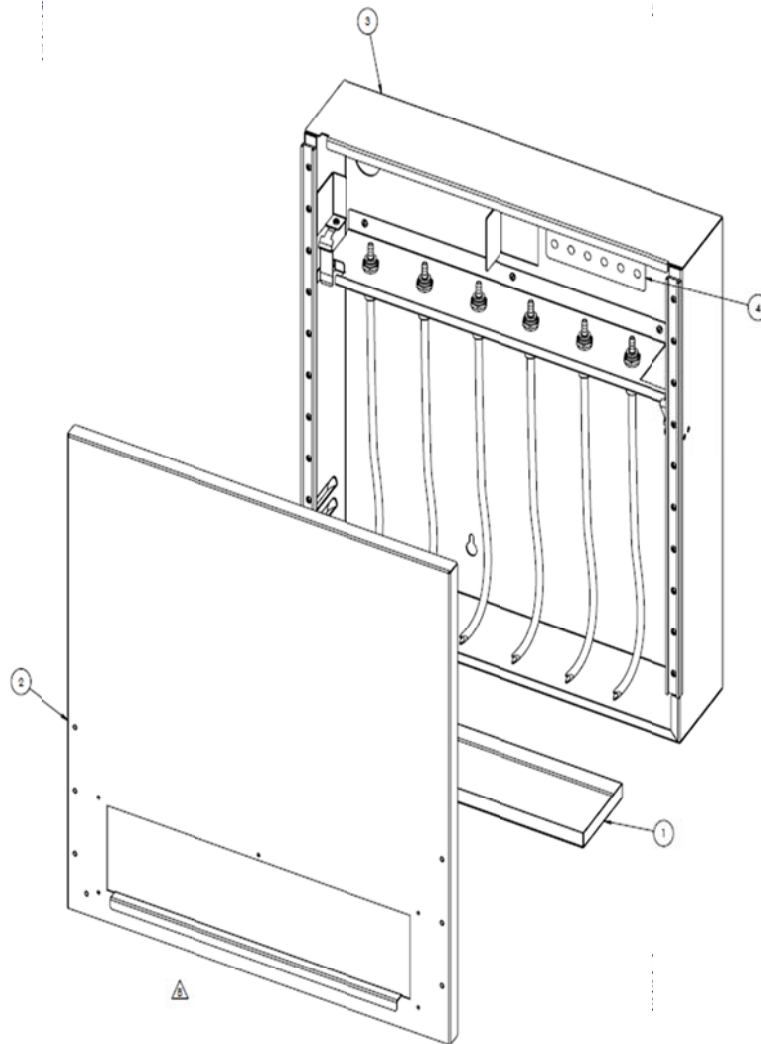
Diagram 22: Delivery System Side Mount Panels
