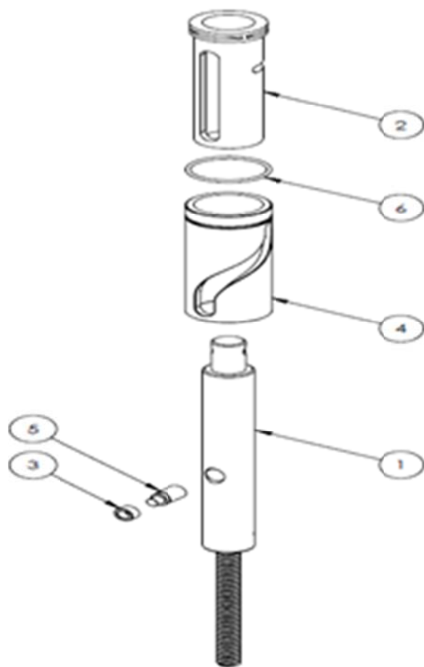
Diagram 13, Assembly Drive Upper Piston
