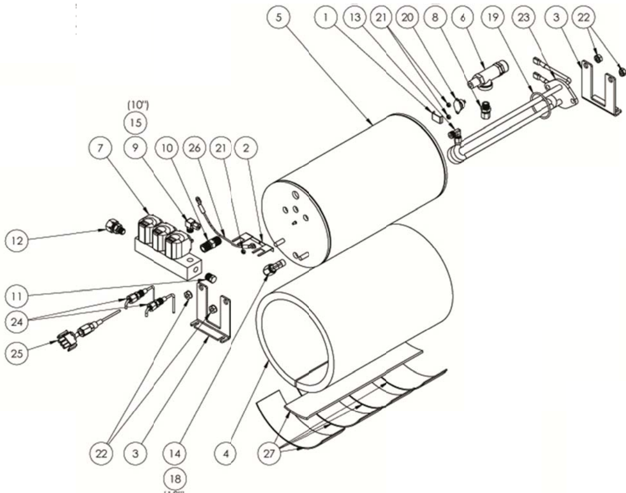
Diagram 25: Steam Tank
