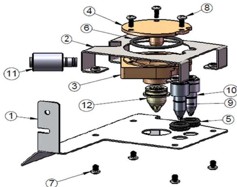
Diagram 8, Parts List: Product Nozzle Non Syrup
