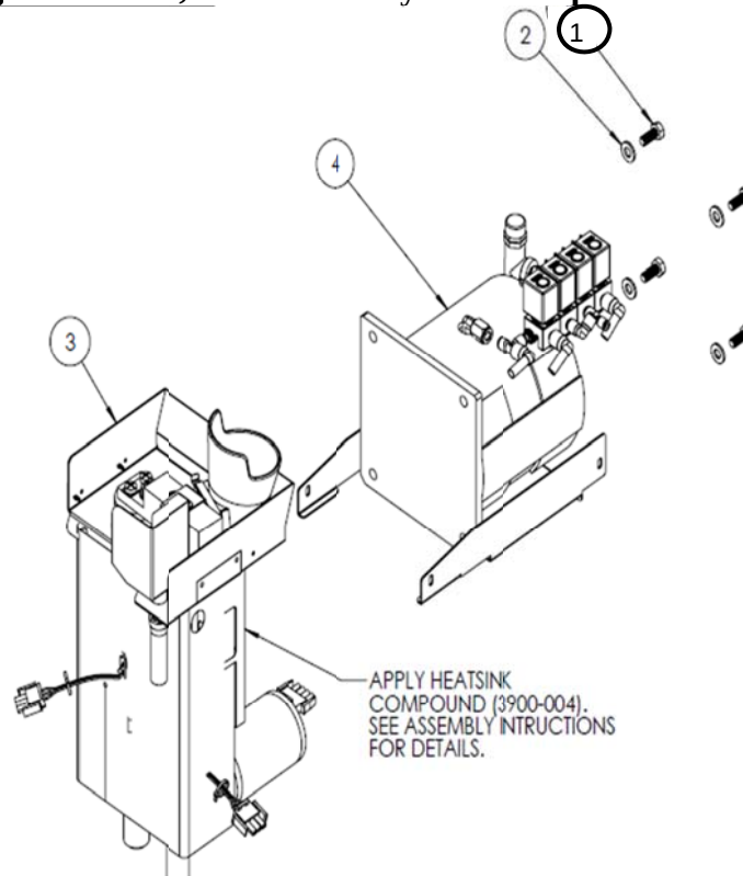
Diagram 10, Assembly Group/Water Tank
