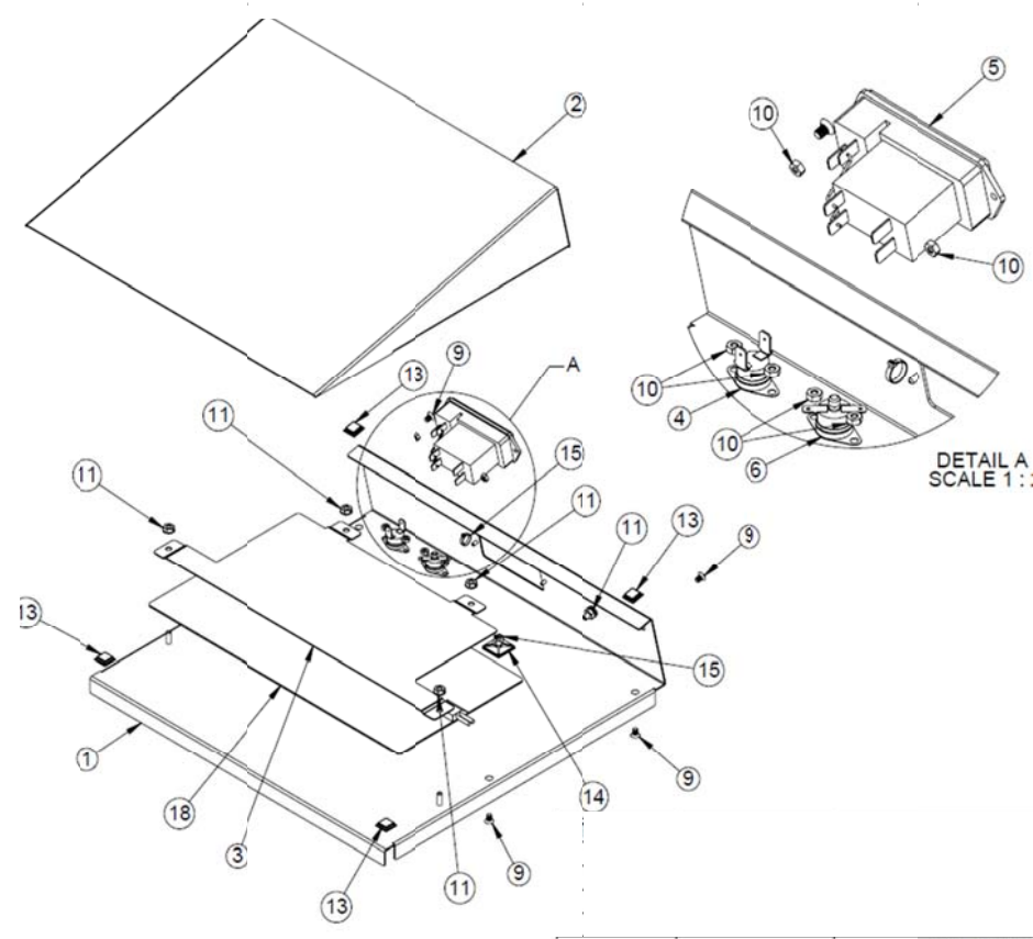
Diagram 20: Assembly Syrup Rack Heater (Bag in a Box)
