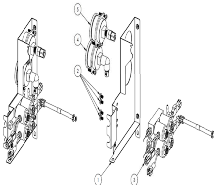
Diagram 21: Water/Steam Gauge/Air Assembly
