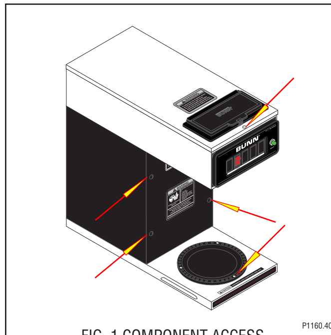
FIG. 1 COMPONENT ACCESS
