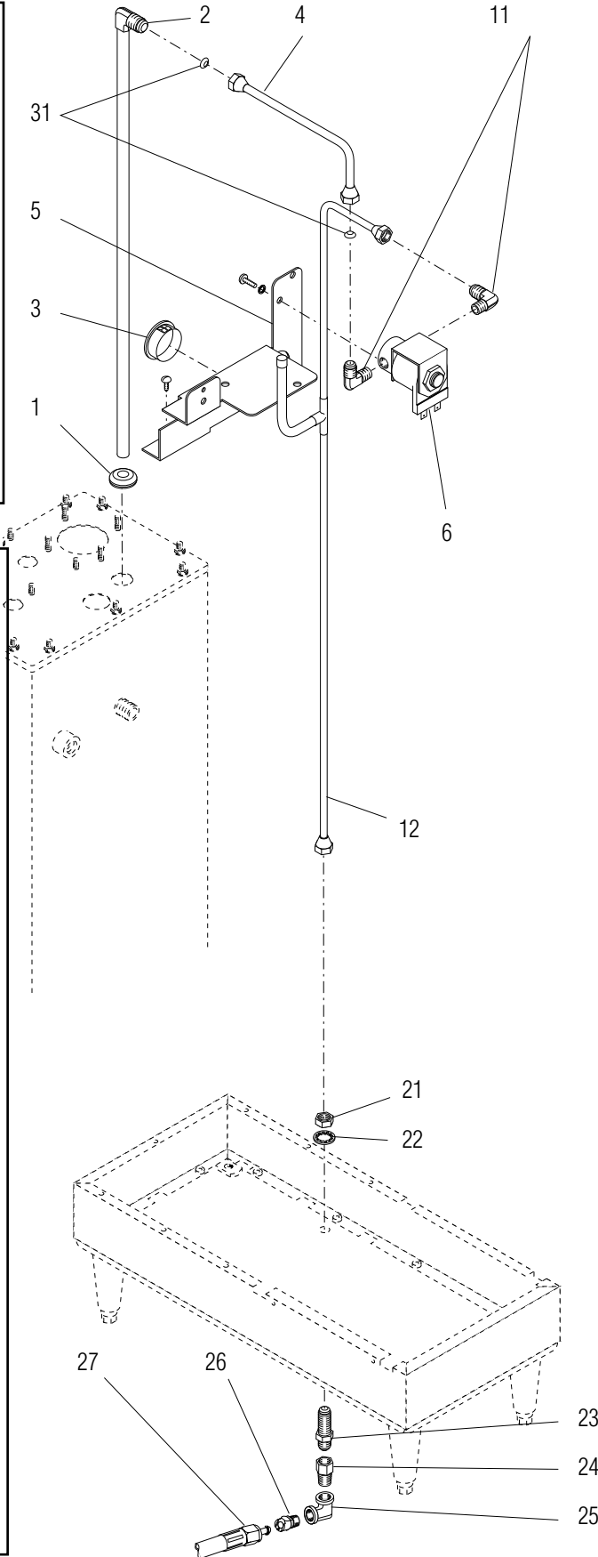
SOLENOID W/1.48" DIA COIL
