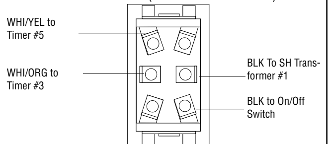
WITHOUT RELAY (After S/N SNG0014000)
