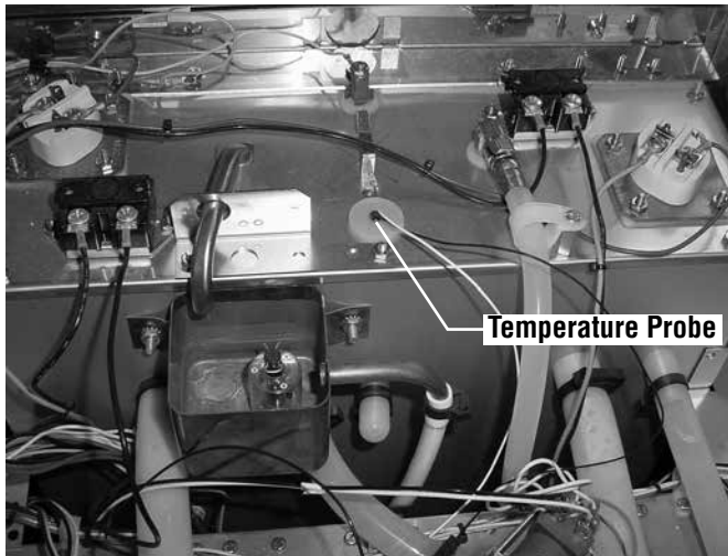
FIG 10 TEMPERATURE PROBE
