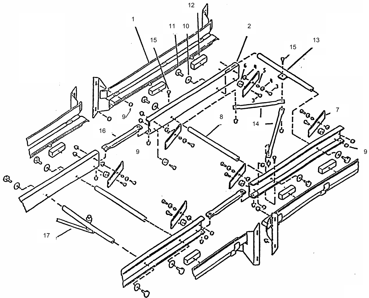
FIGURE: 15. RACK CONVEYOR ASSEMBLY
