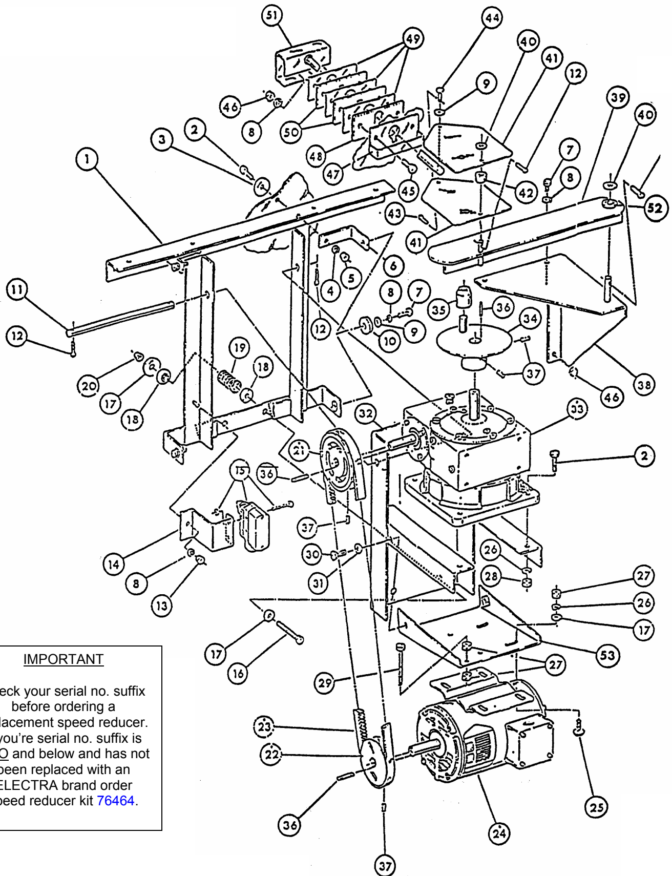
FIGURE: 14. TYPE "D" DRIVE ASSEMBLY
