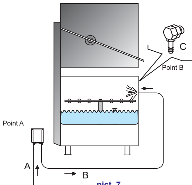
pict. 7 CONNECTION DIAGRAM
