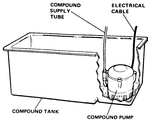
Figure 2-10. Compound Pump Installed In Tank
