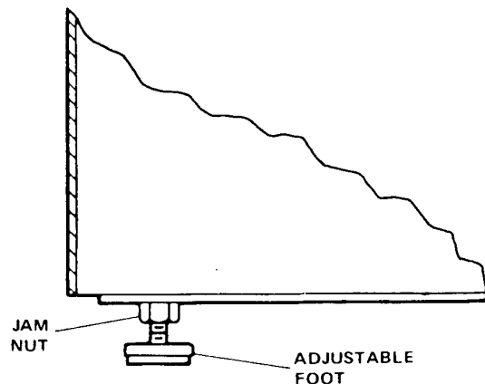
Figure 2-7. Adjustable Foot (Model BB1224)
