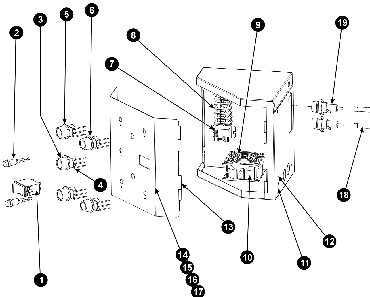
Figure "H" Electric Control Box
