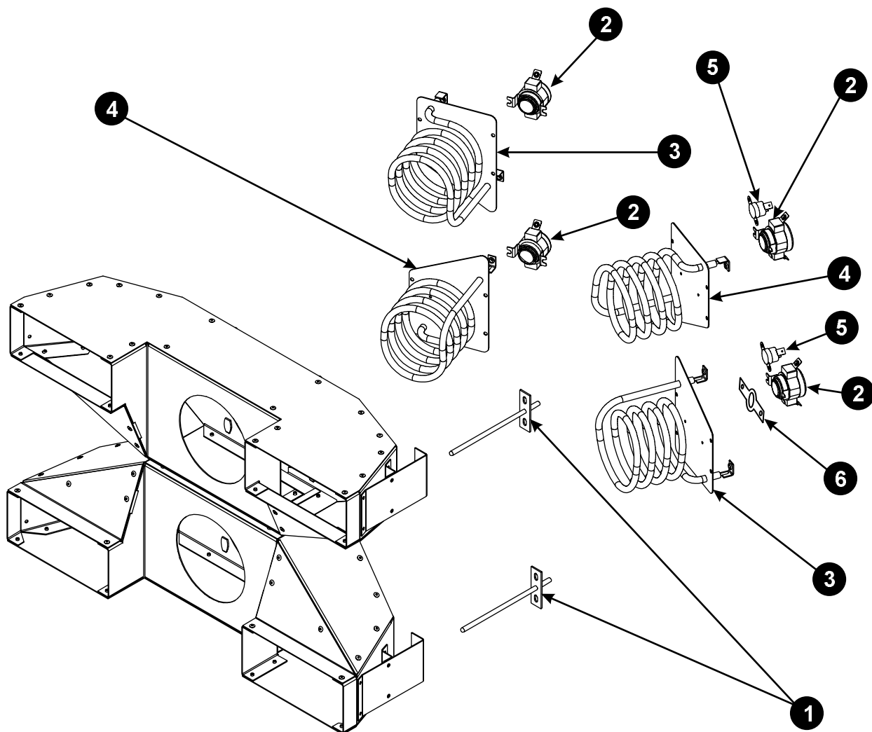
Figure “I” Cool-Down Thermostat, Elements, Switch & Probe
