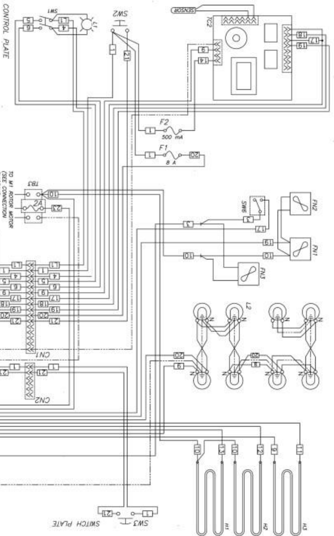
LADDER DIAGRAM
