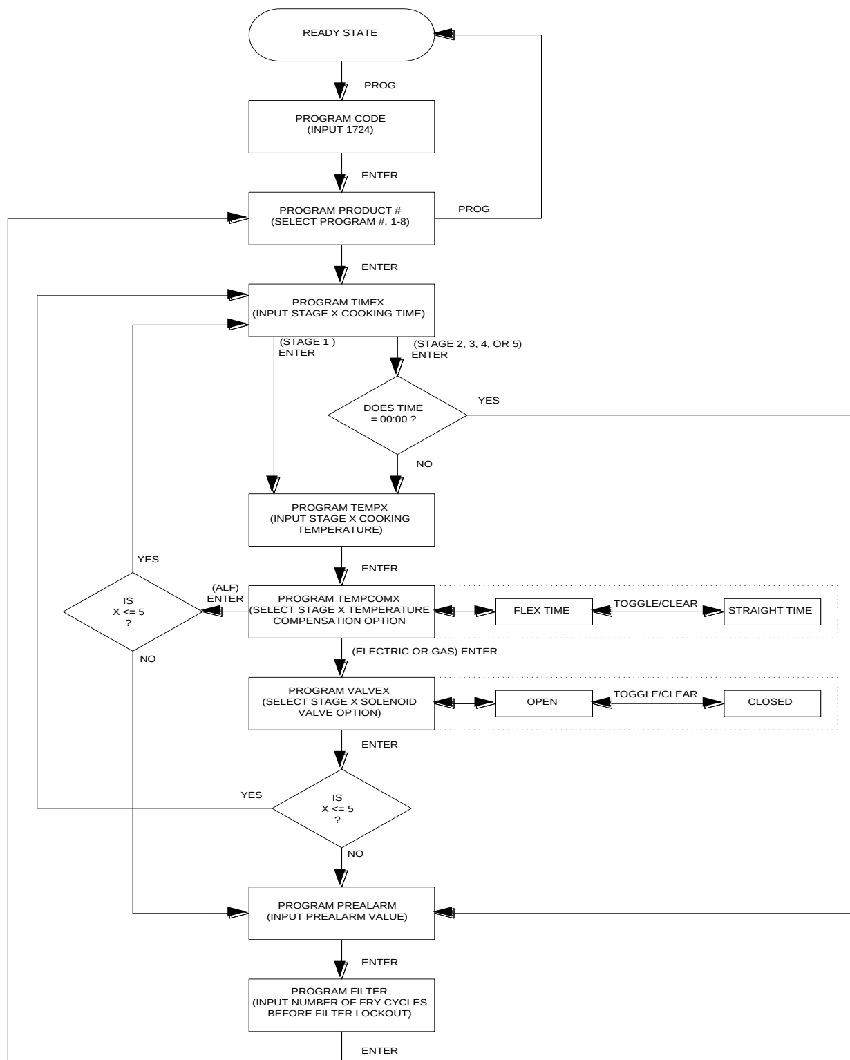
Figure 2. Product Programming Sequence
