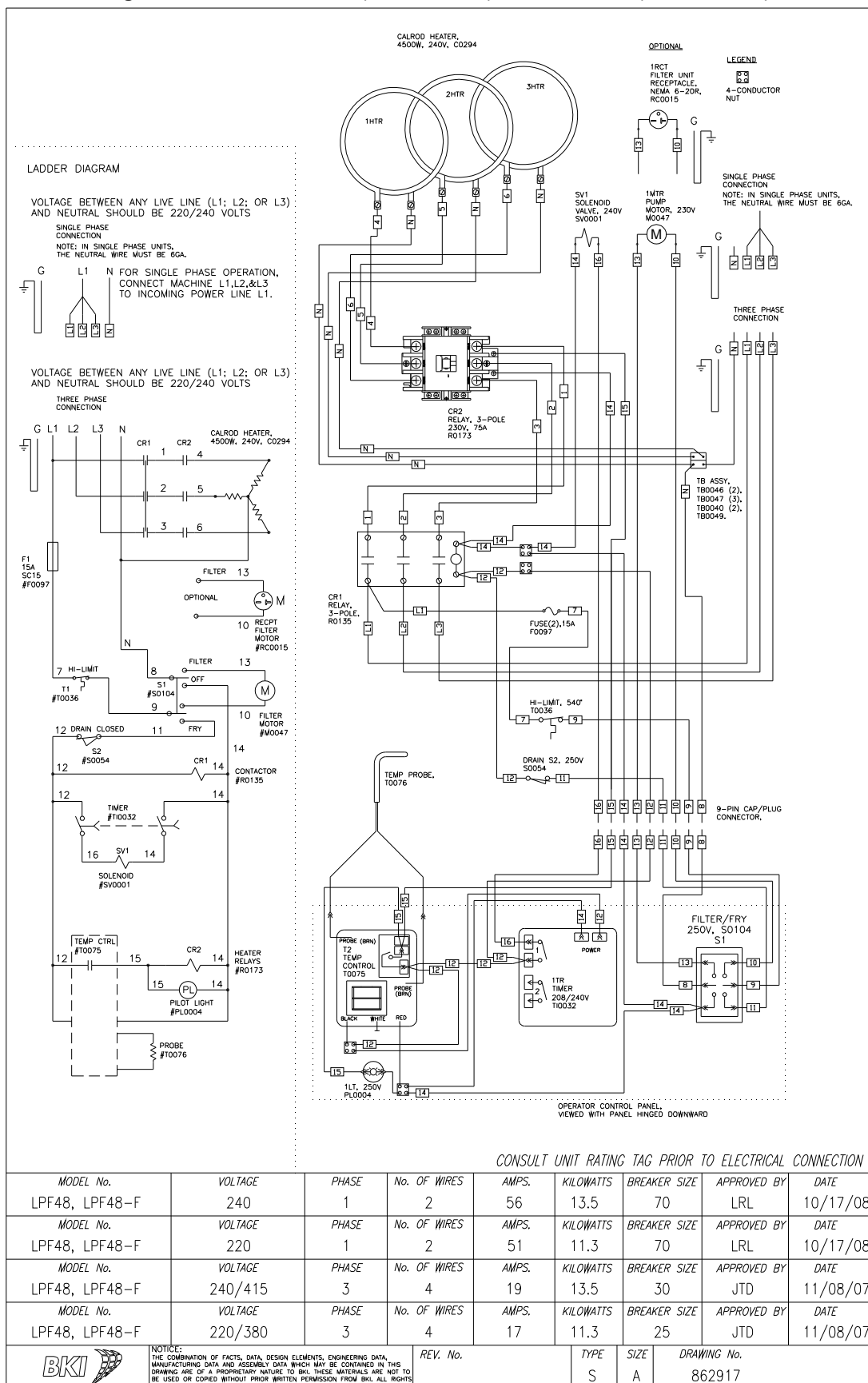
Figure 17. LPF 220V/380V(1 or 3 Phase) or 240V/415V (1 or 3 Phase)
