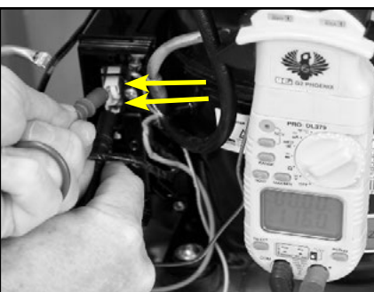
1. Check for 80-120VAC at the white and black wires entering the Inverter.
