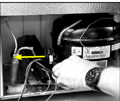
7. Using a pry tool, pull the plug and ground wire from the compressor. Note the orientation of the plug before removing.
