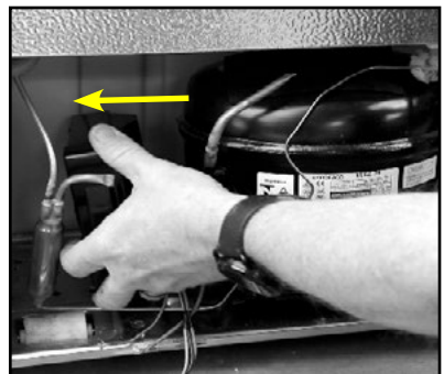
6. Pull the inverter off of the side of the compressor.
