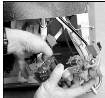
3. Unplug the harnesses from the water valve.
