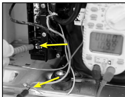
2. Check for 80-120VAC between the thin single black wire entering the Inverter and the cabinet.
