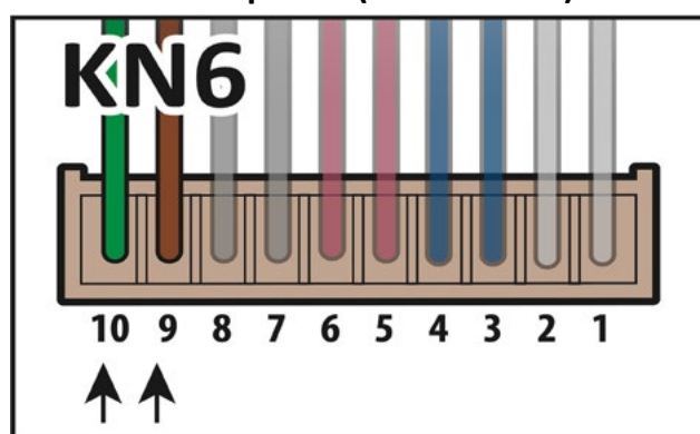
E8 Test points (Ice Maker 2 )
