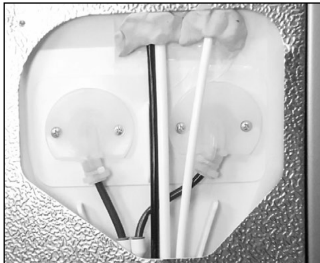
Fill Tube Heaters & Water Lines
