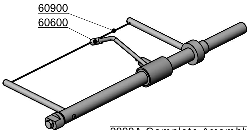
3800A Complete Assembly
