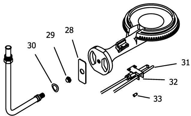
LP GAS (CX) BURNER ASSEMBLY
