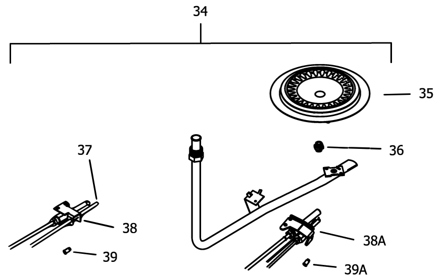
LP GAS (SX) BURNER ASSEMBLY
