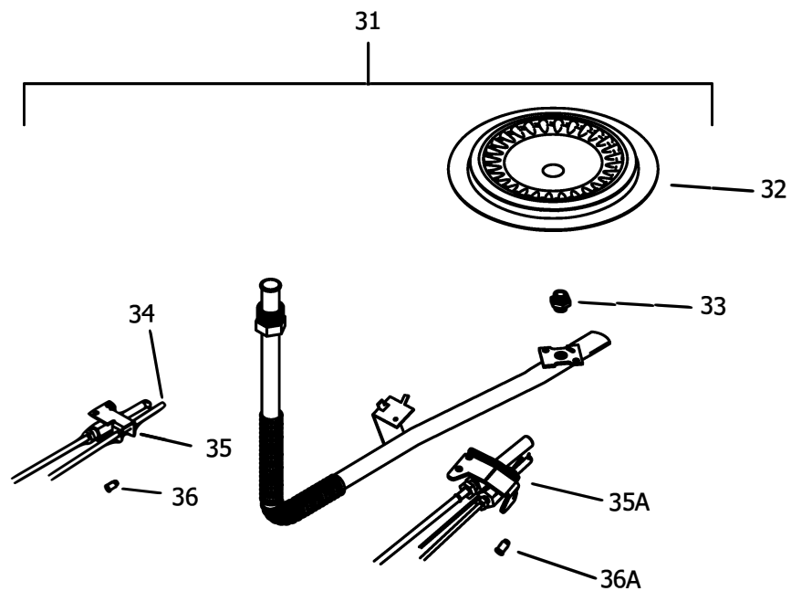
LP GAS (SX) BURNER ASSEMBLY
