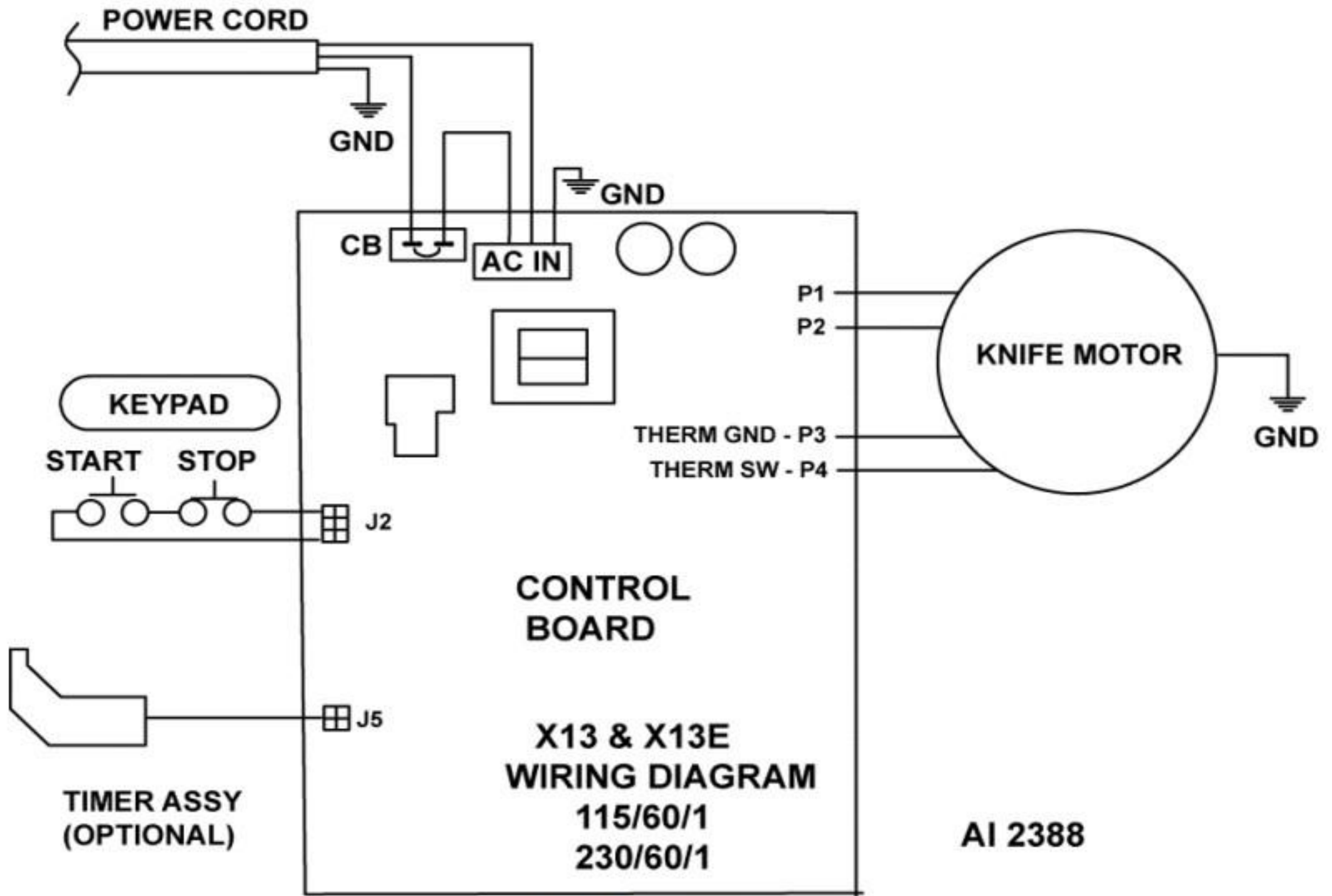
X13 & X13E Wiring Diagram
