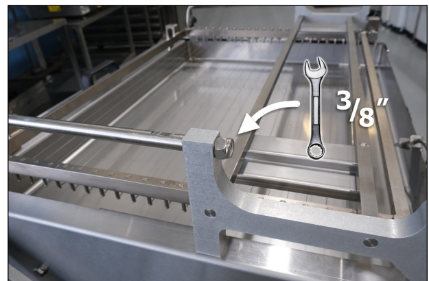
Figure 4: Removing the Tray Retainer Handle.
