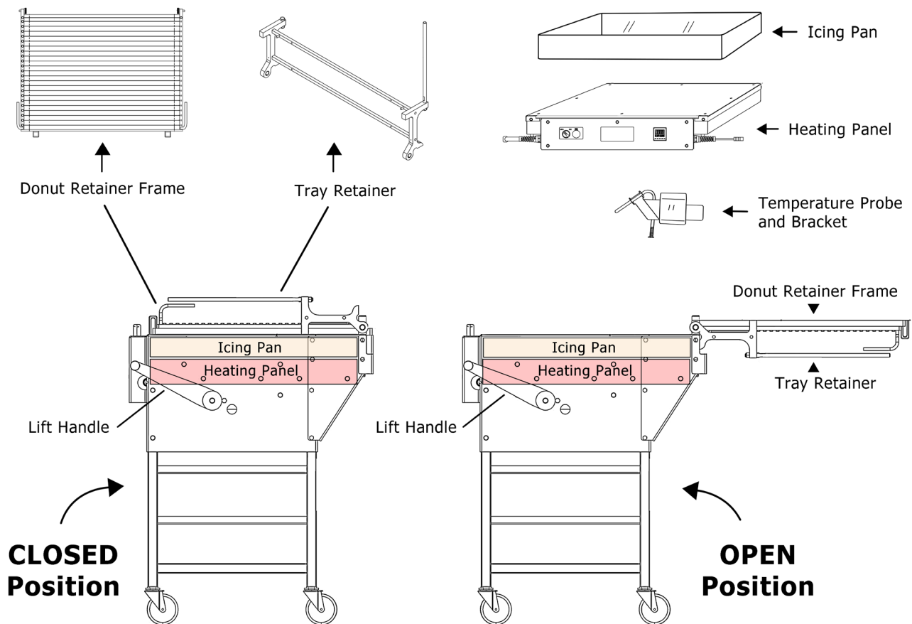
Figure 1: Main parts of the HI18/24 Icer showing OPEN and CLOSED position
