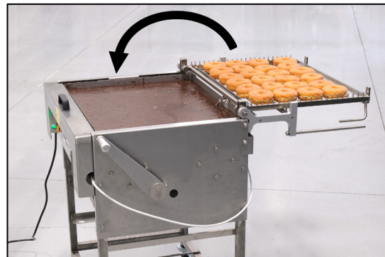
Figure 8: Rotate to CLOSED position.
