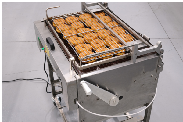
Figure 13: Donut Retainer Frame.
