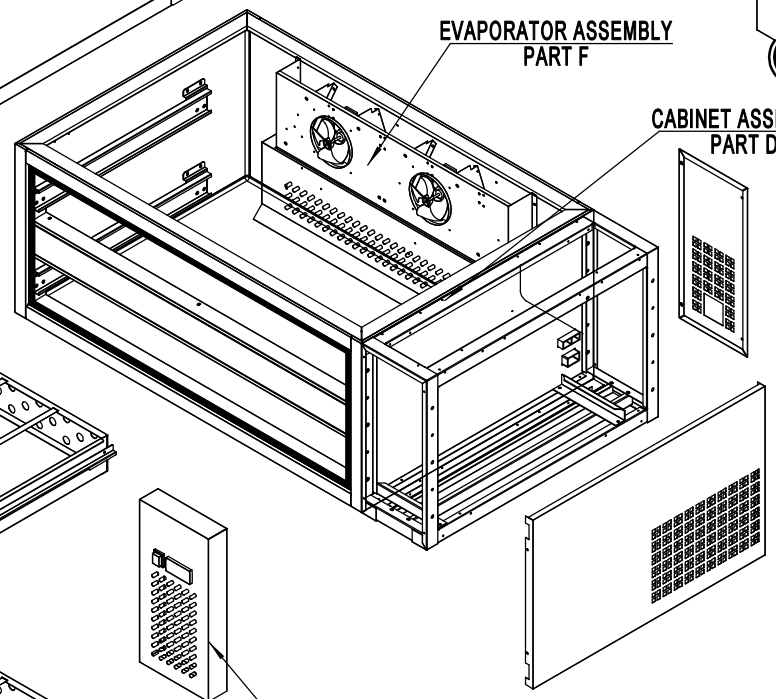
UNIT FRONT ASSEMBLY PART C
