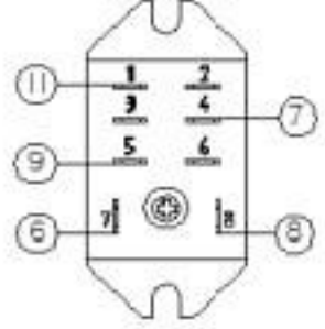
ALTERNATE RELAY WIRING
