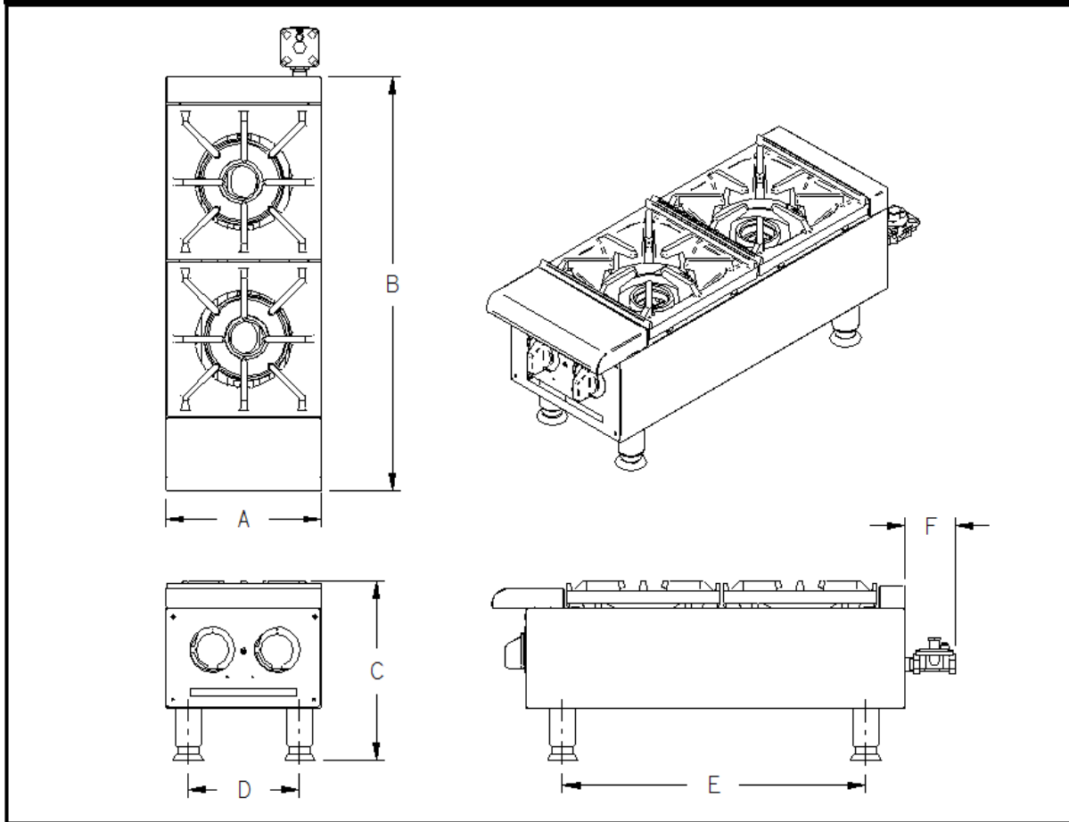
DIMENSIONS - (GHP-2i SHOWN FOR CLARITY)
