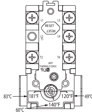
Figure 3. A-8 Thermostat
