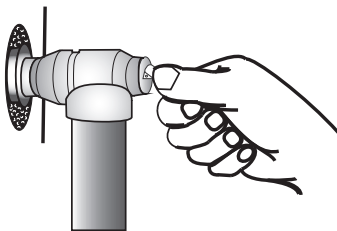
Figure 6. Testing the Temperature-Pressure Relief Valve
