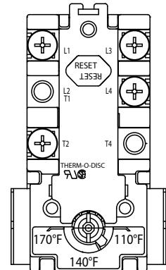
Figure 4. C-2 Thermostat
