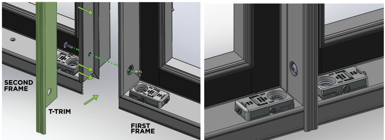
Figure 2.8: T-Trim installation
