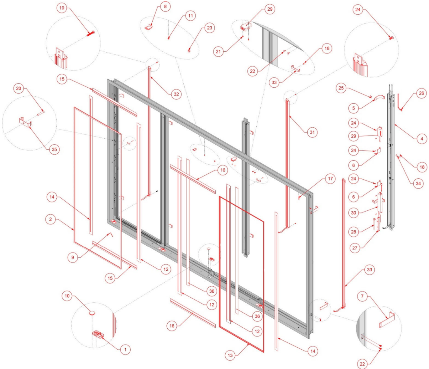
Figure 9.1 Frame Assembly for Vista C Series Normal Temperature for Replacement Parts (See Table 9.1 for Part Numbers)
