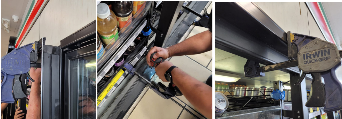
Figure 2.2: Clamps to insert Frame into Net Opening
