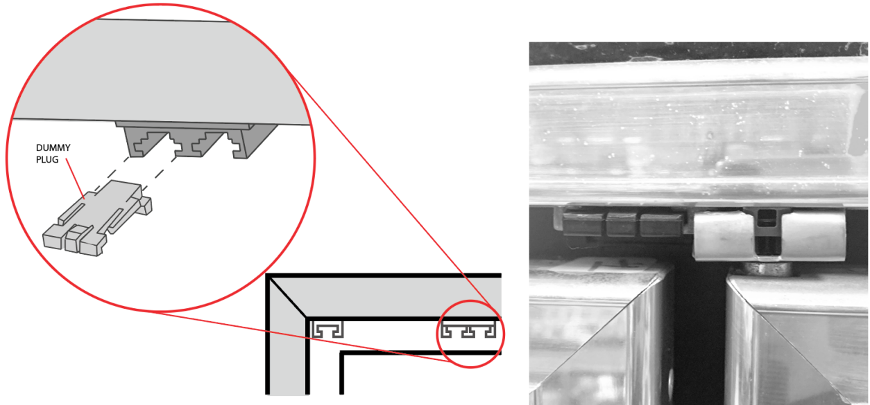
Figure C.2: Plug Removal
