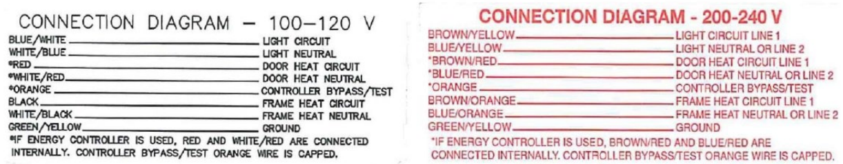
Figure 2.11: Wiring Labels
