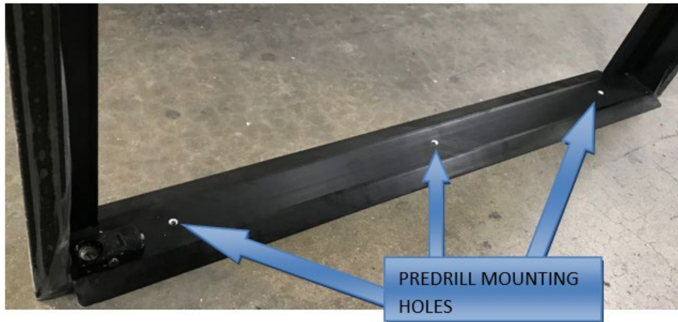
Figure 17.4: Mounting Holes
