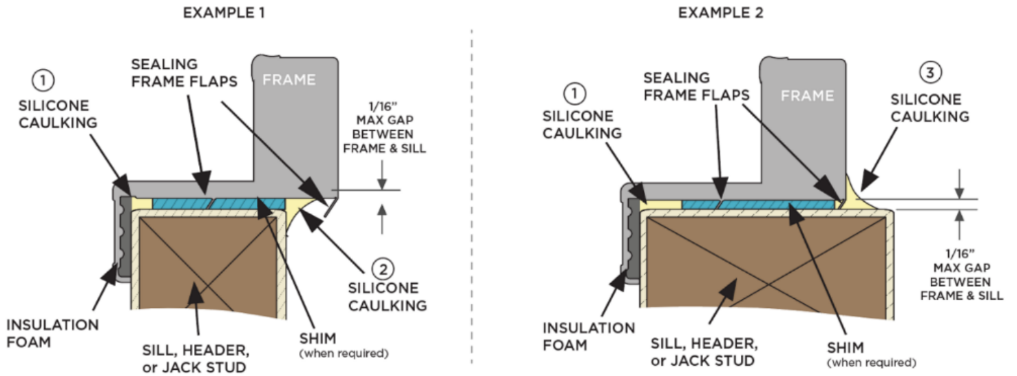
Figure 17.2: Frame Shimming and Sealing Details
