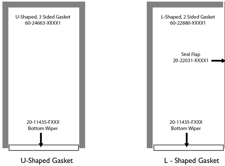
Figure 20.2 Door Assembly for Infinity 90 Series NT Pass-Thru; Replacement Parts
