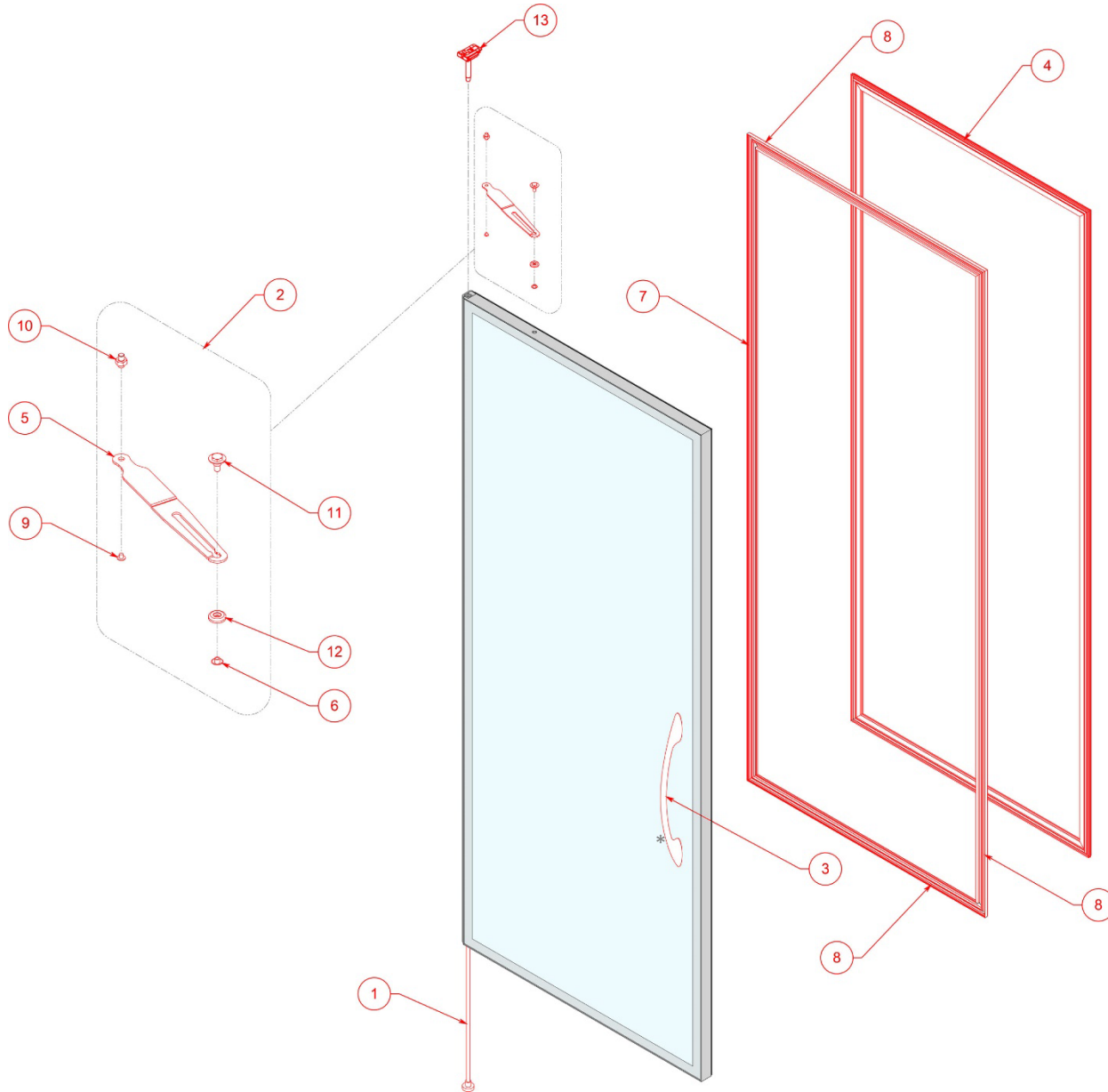
Figure 10.1 Door Assembly for Infinity 90 Series Door, for Replacement Parts
