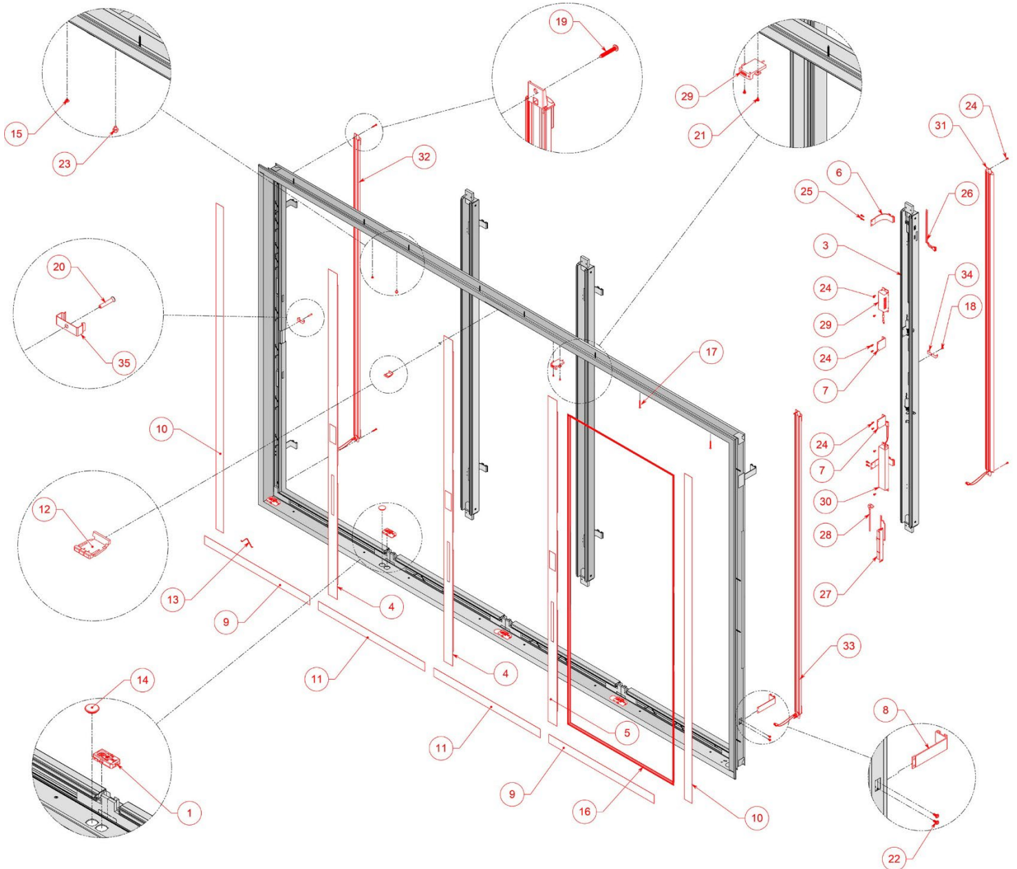
Figure 9.1 Frame Assembly for Infinity 90 Series Normal and Low Temperature for Replacement Parts
