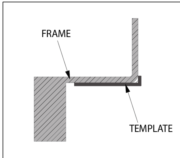
Figure E.3: Template Placement on Frame Side view
