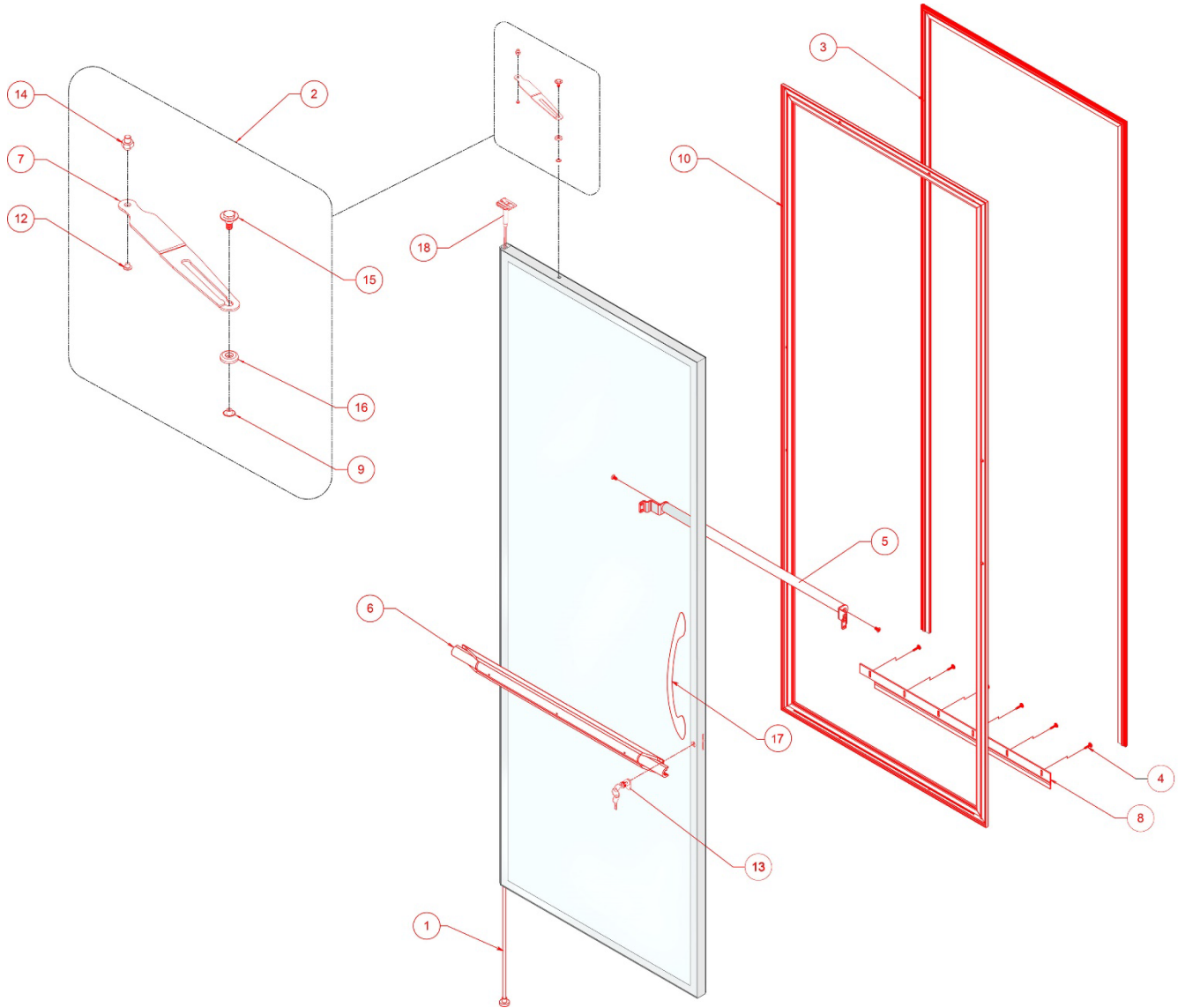
Figure 20.1 Door Assembly for Infinity 90 Series NT Pass-Thru; Replacement Parts
