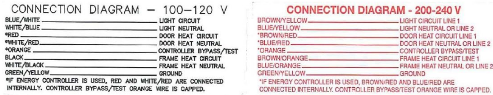
Figure 17.7: Wiring Labels
