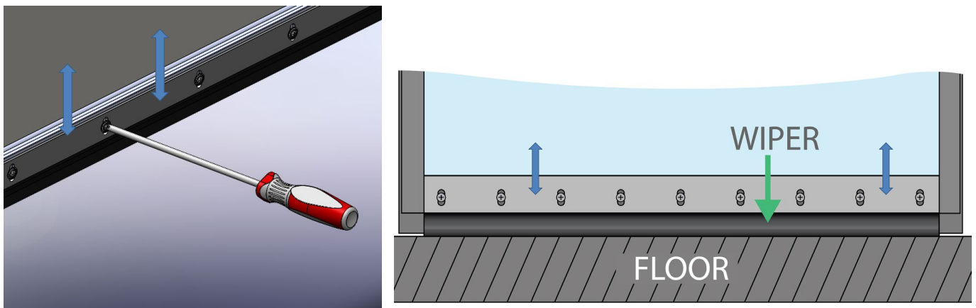
Figure I.1 – Wiper Adjustment
