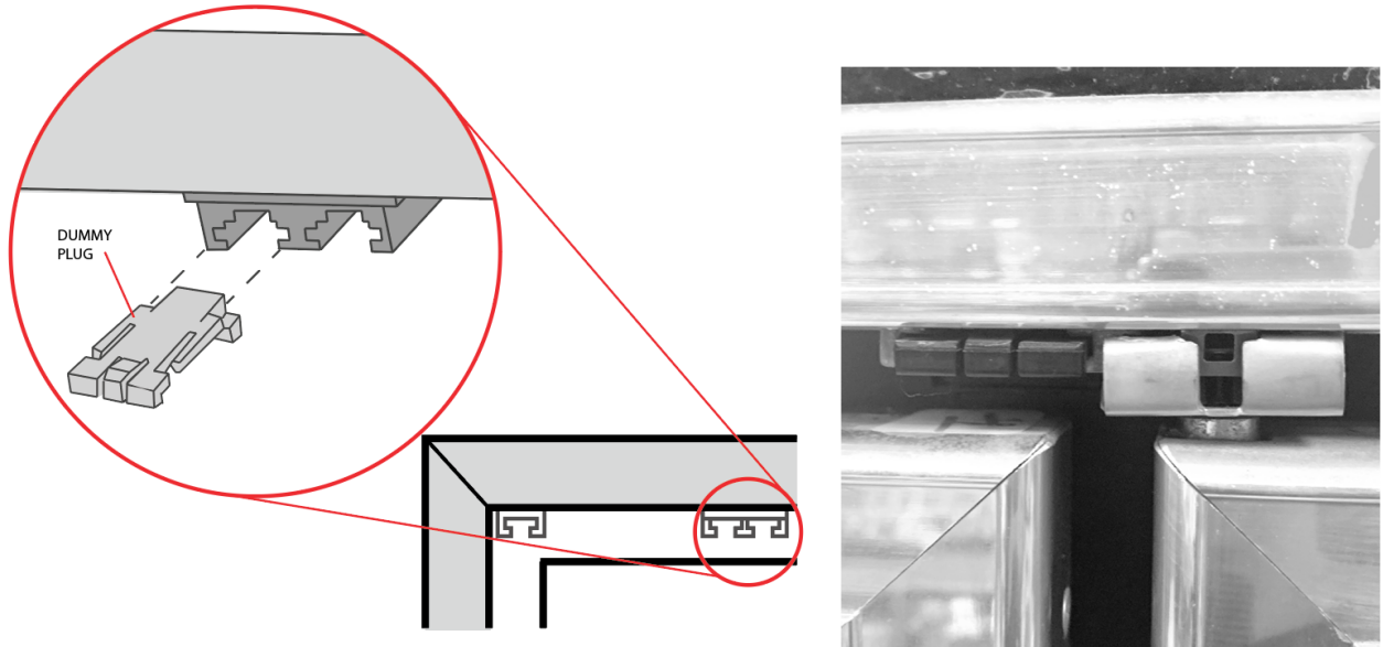
Figure C.2: Plug Removal
