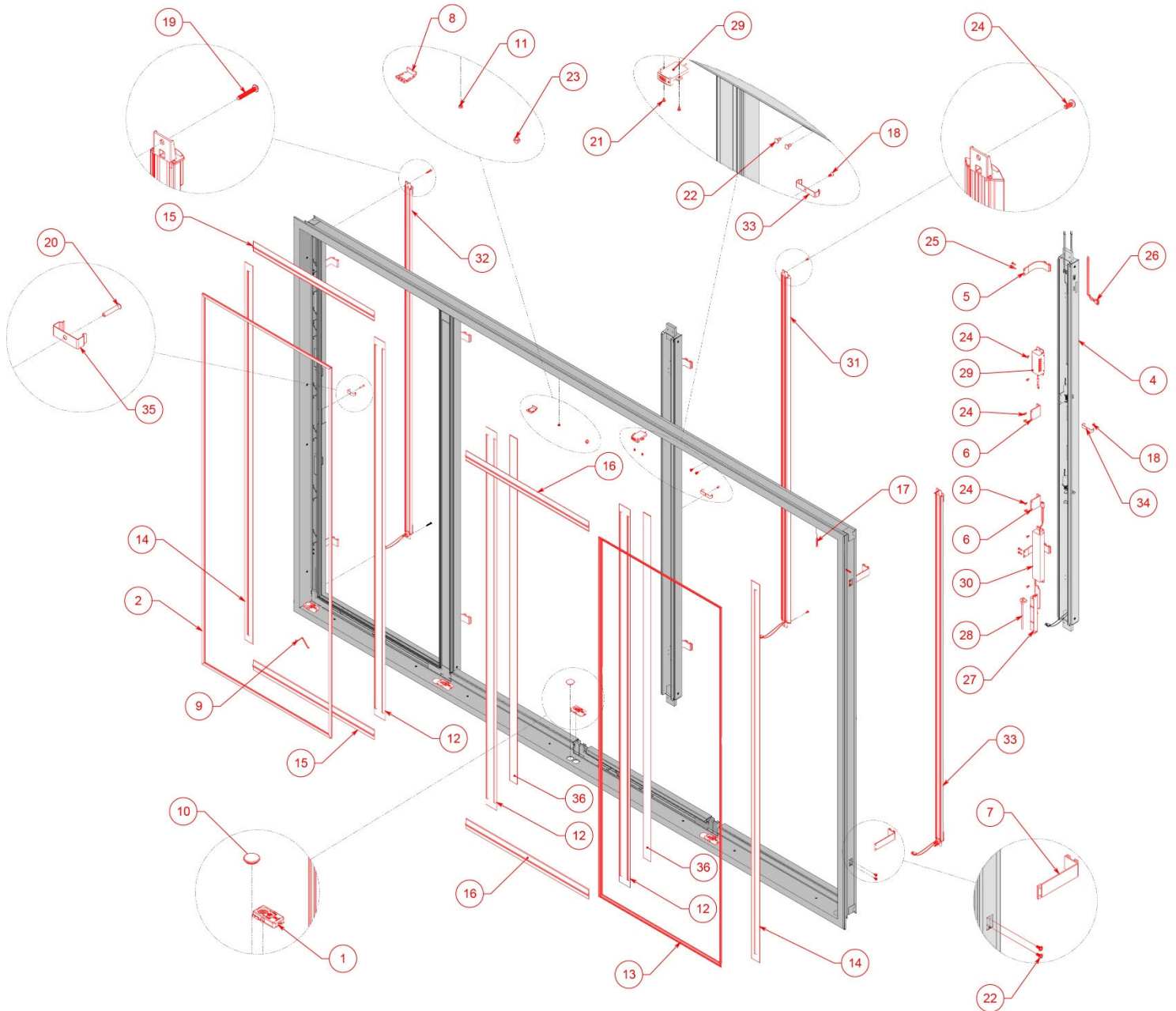
Figure 9.1 Frame Assembly for Infinity 60 Series Normal Temperature for Replacement Parts
