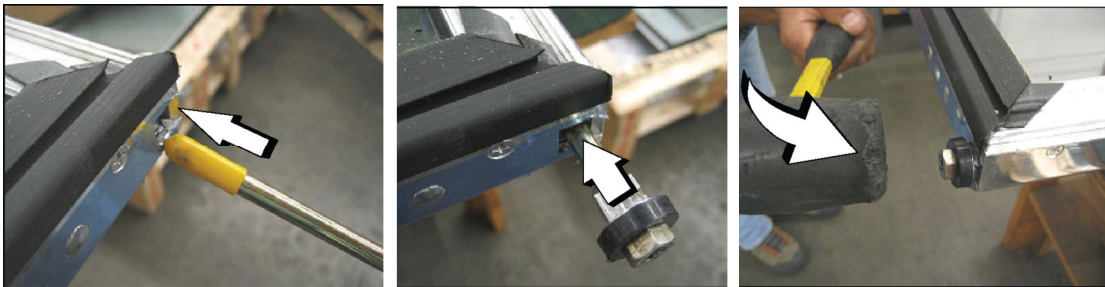
Figure 12.3 Removing torque rod from the door.
