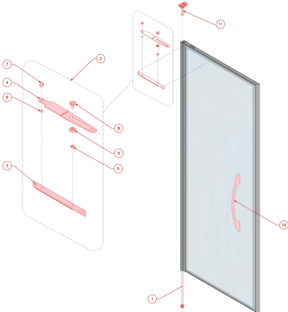
Figure 10.1 Door Assembly for Infinity 60 Series Door, for Replacement Parts
