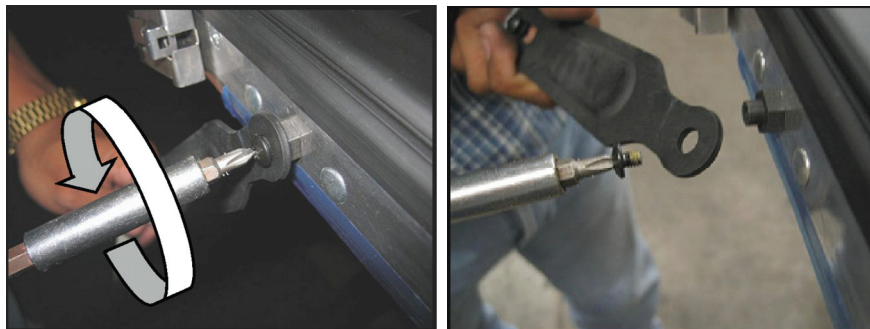
Figure 14.1 Removing hold-open assembly from door.
