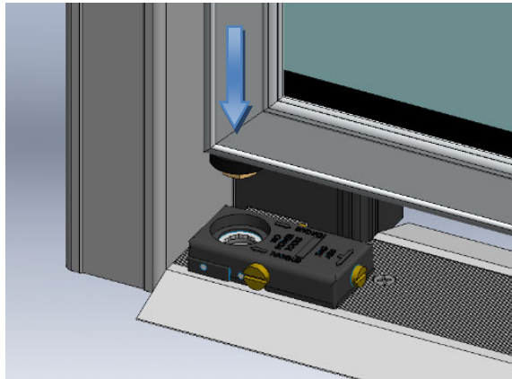
Figure 18.1: Inserting door Torque Rod into TorqueMaster
