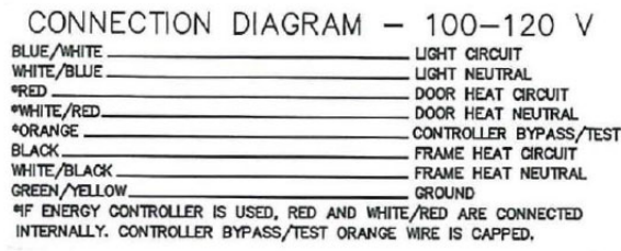
Figure 2.11: Wiring Labels
