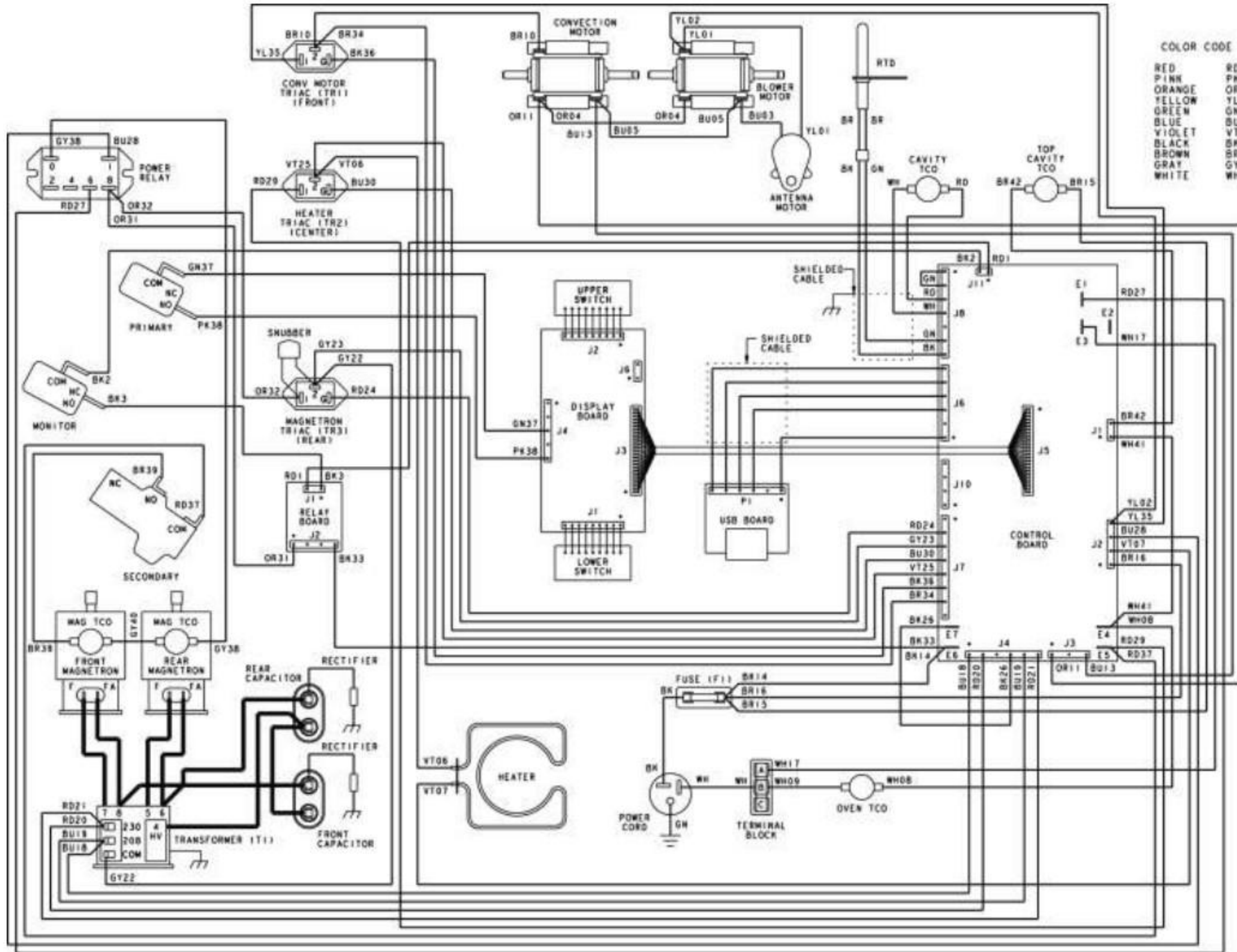
WIRING DIAGRAM
