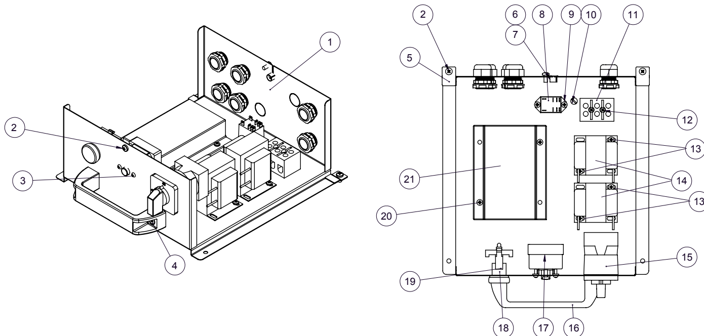
120V CONFIGURATION REFERENCE DRAWING 5014823
