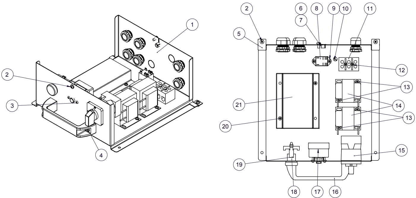
120V CONFIGURATION REFERENCE DRAWING 5014823
