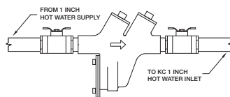
Backflow Preventer
