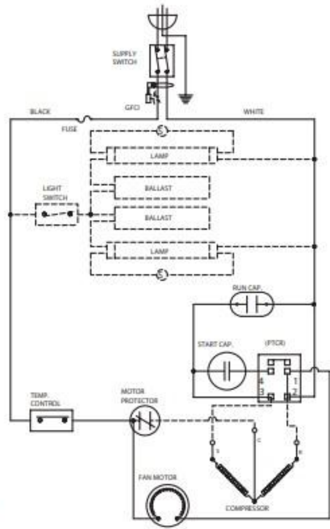
WIRE DIAGRAM 00-C-2030-00 F
