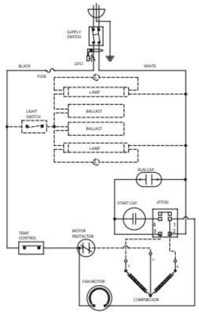
WIRE DIAGRAM 00-C-2030-00 F
