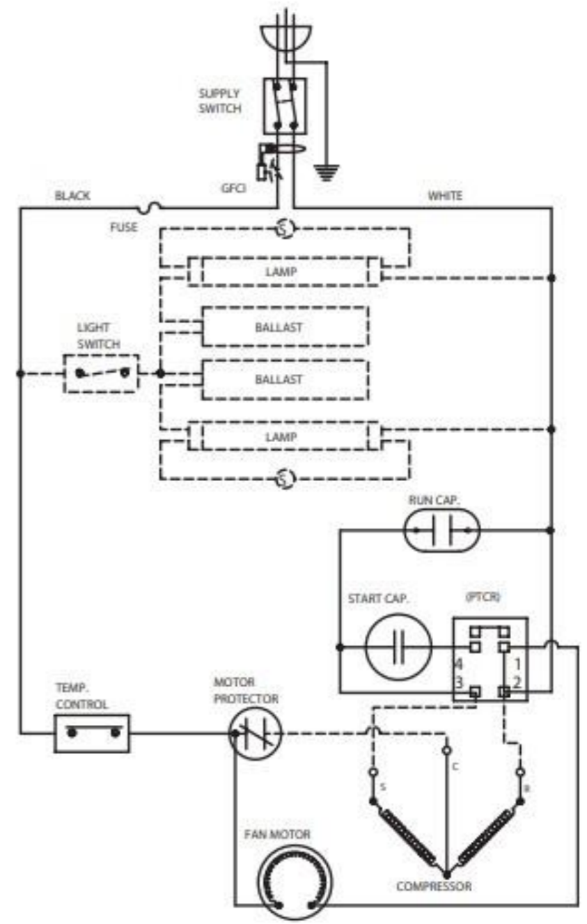
WIRE DIAGRAM 00-C-2030-00 F
